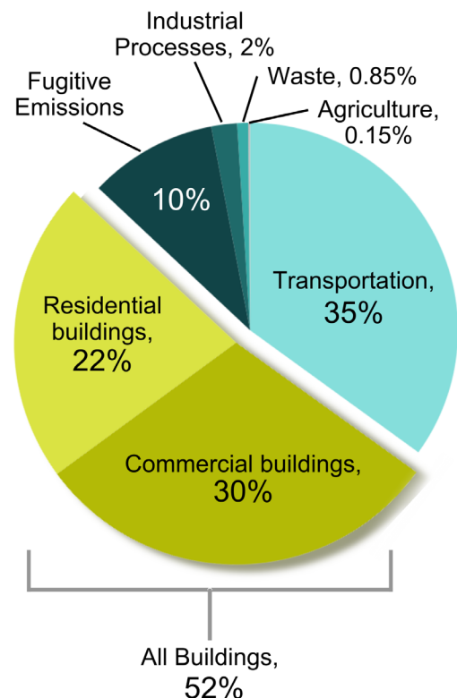
Figure 2: Share of regional climate pollution broken out by sector.
